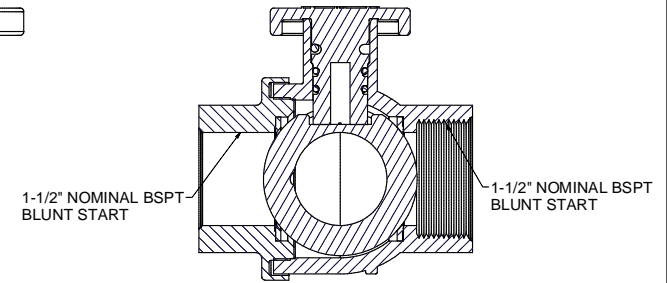
SECTION B-B SCALE 1 : 1
